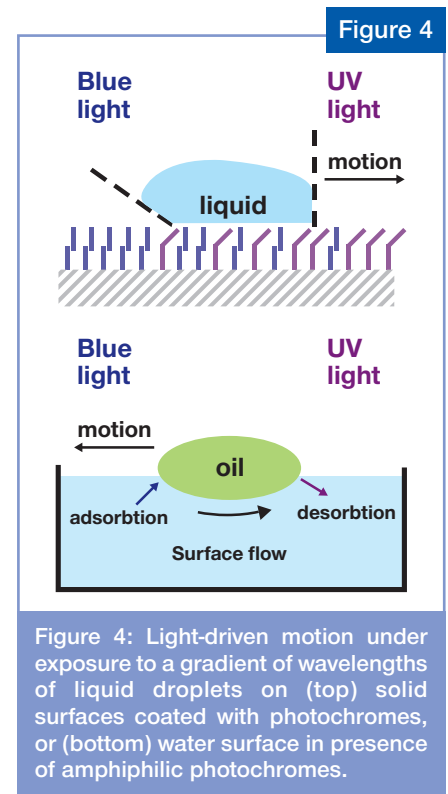
Figure 4: Light-driven motion under exposure to a gradient of wavelengths of liquid droplets on (top) solid surfaces coated with photochromes, or (bottom) water surface in presence of amphiphilic photochromes.
